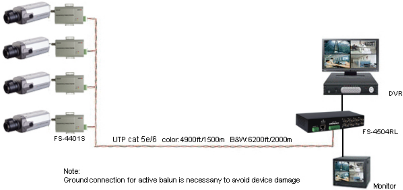
Diagram 3 FS-4401S + FS-4504RL
